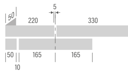
330 x 50 x 12 mm cross bond 1/2
