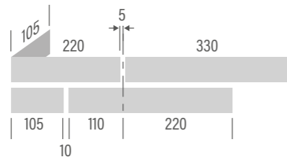
330 x 50 x 12 mm cross bond 1/3
