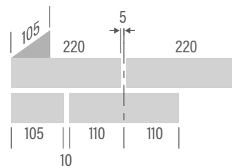
215 x 65 x 12 mm cross bond 1/2
